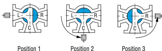
Arrangement 7: 3-way, 3-port, 180° Turn – Three Positions
