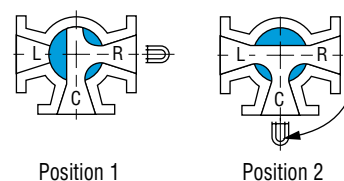
Arrangement 6: 3-way, 3-port, 90° Turn – Two Positions
