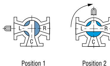
Arrangement 5: 3-way, 3-port, 90° Turn – Two Positions
