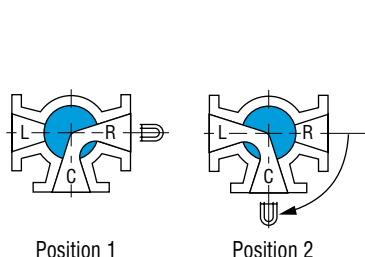
Arrangement 1: 3-way, 2-port, 90° Turn – Two Positions
