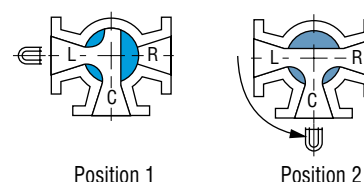
Arrangement 3: 3-way, 3-port, 90° Turn – Two Positions
