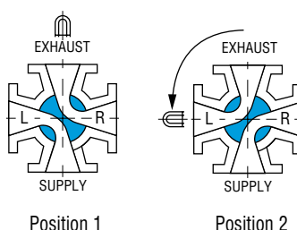
Arrangement 2: 4-way, 4-port, 90° Turn – Two Positions
