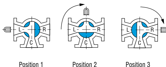
Arrangement 8: 3-way, 3-port, 180° Turn – Three Positions
