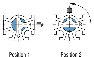
Arrangement 4: 3-way, 3-port, 90° Turn – Two Positions
