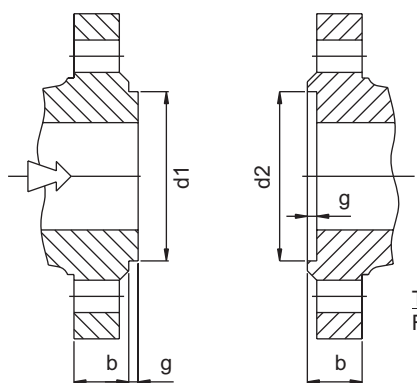
TYPE V 13 - Male-faced according to DIN 2513
