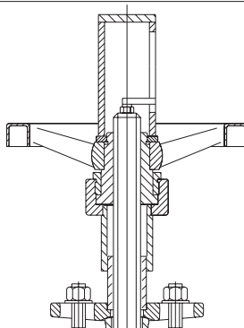
⑪ Position indicator with stem protection
