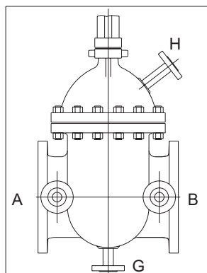
48 Flanges connection
