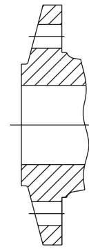
TYPE M - Bevel for diaphragm seal welding according to DIN 2695
