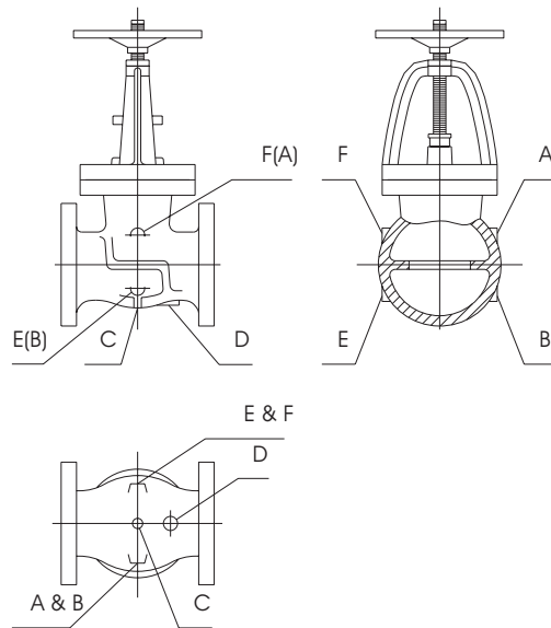
GLOBE VALVE
