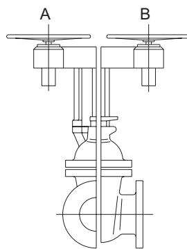
③ Bevel gearing with horizontal handwheel
