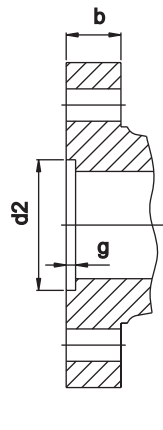
TYPE R 14 - Female-facing according to DIN 2514
