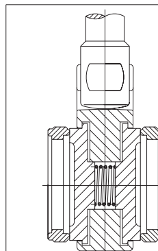
28 Parallel disk
