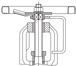
⑨ Position indicator for globe valve
