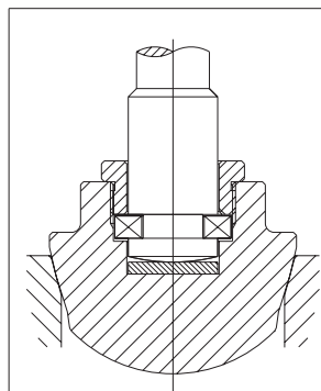
36 Parabolic / regulating disk
