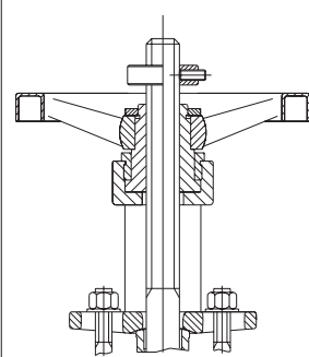
⑯ Travel limit
