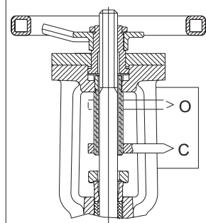
⑧ Position indicator
