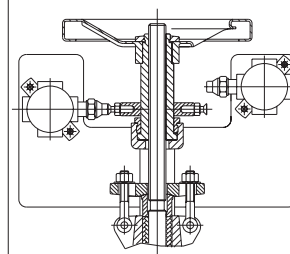
⑫ Position indicator with limit switches
