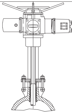
⑥ Electric actuator
