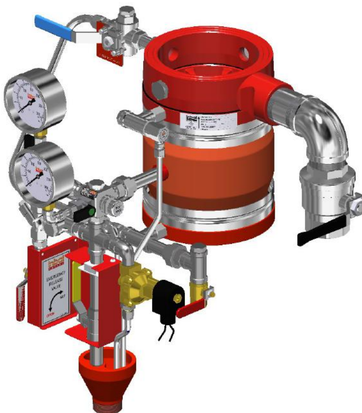
Model 799DX-04C01
