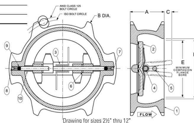
KW-900-W Wafer
